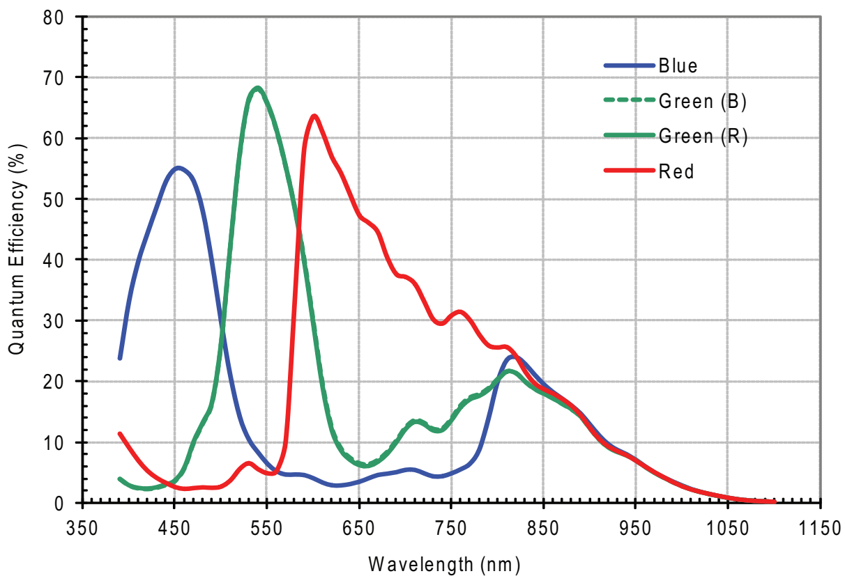
Figure 8: Quantum Efficiency
