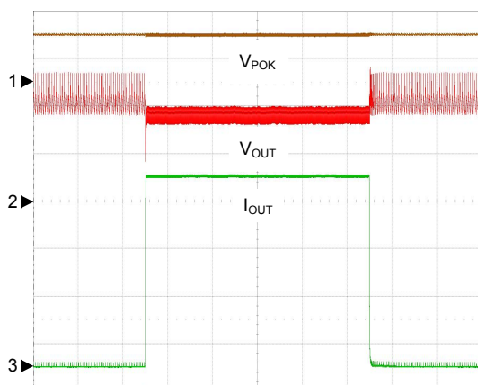
Load Transient
