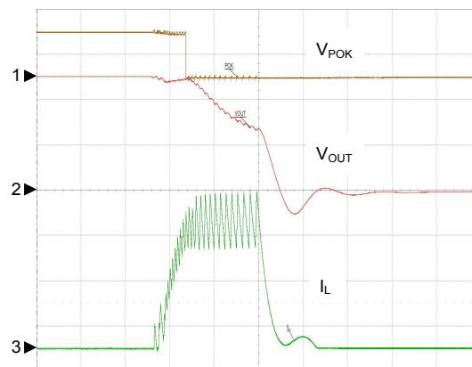
Current Limit
