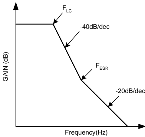
Figure 3. The LC Filter GAIN and Frequency
