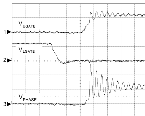
UGATE Rising
