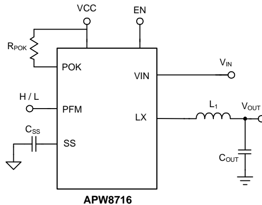
APW8716
