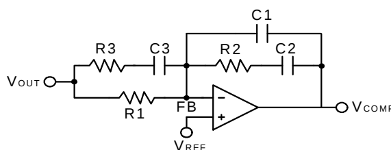
Figure 6. Compensation Network
