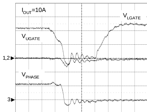
UGATE Falling
