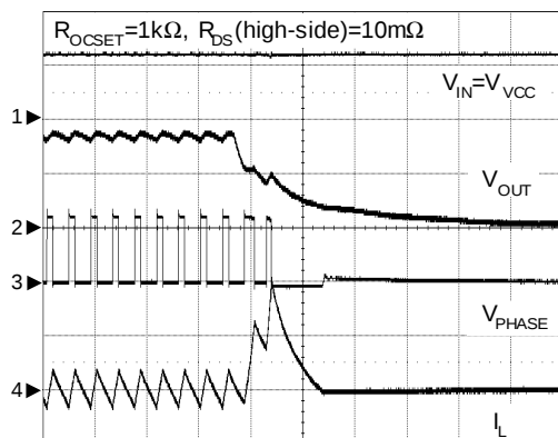
Short-Circuit Protection
