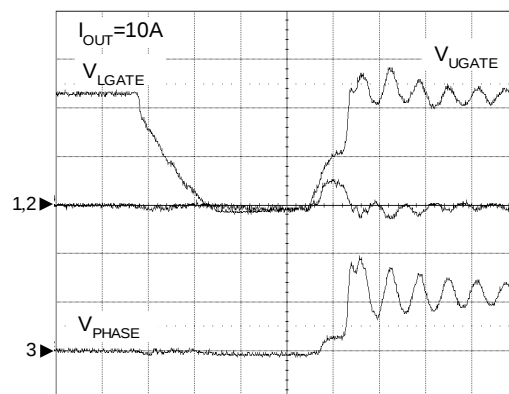
UGATE Rising
