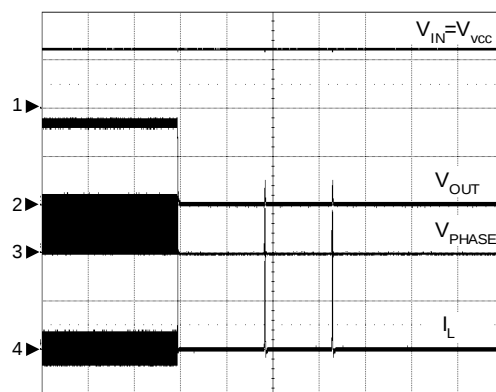
Over-Current Protection
