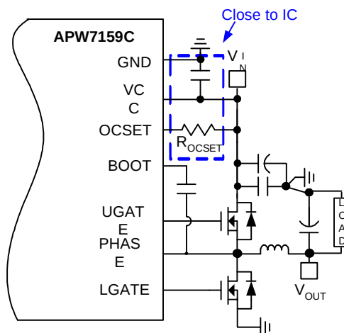
Figure 8. Layout Consideration
