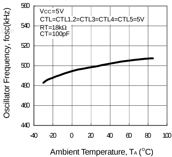
Oscillator Frequency vs. Ambient Temperature
