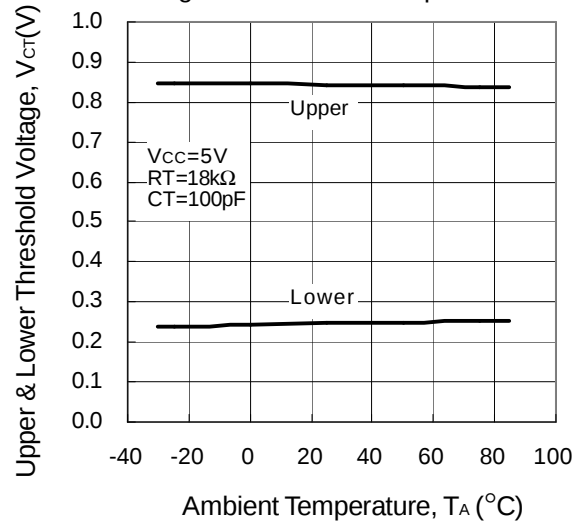
Triangular Wave Upper & Lower Threshold Voltages vs. Ambient Temperature
