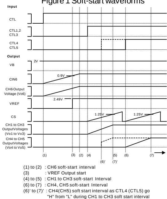
Figure 2 Soft-start waveforms
