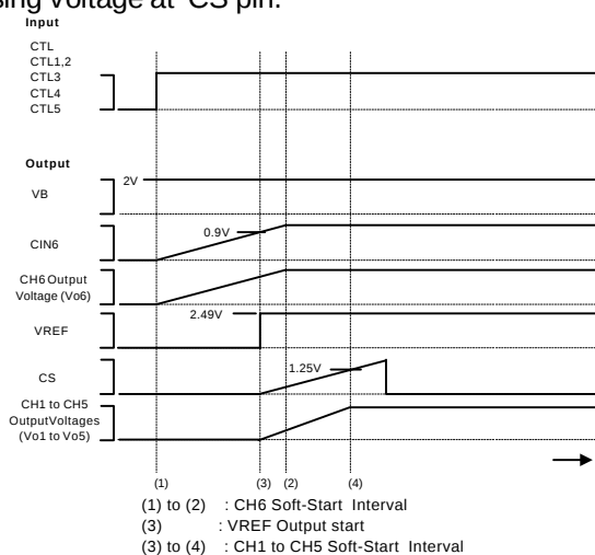
Figure 1 Soft-start waveforms
