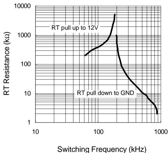
RT Resistance vs. Switching Frequency
