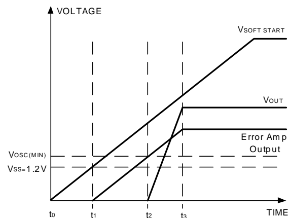
FIGURE 1. SOFT-START INTERVAL
