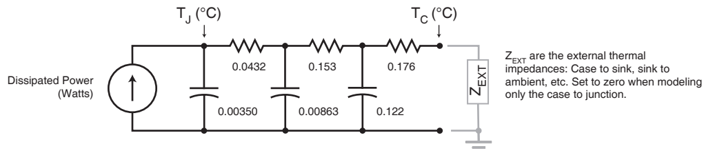
Figure 11, Transient Thermal Impedance Model
