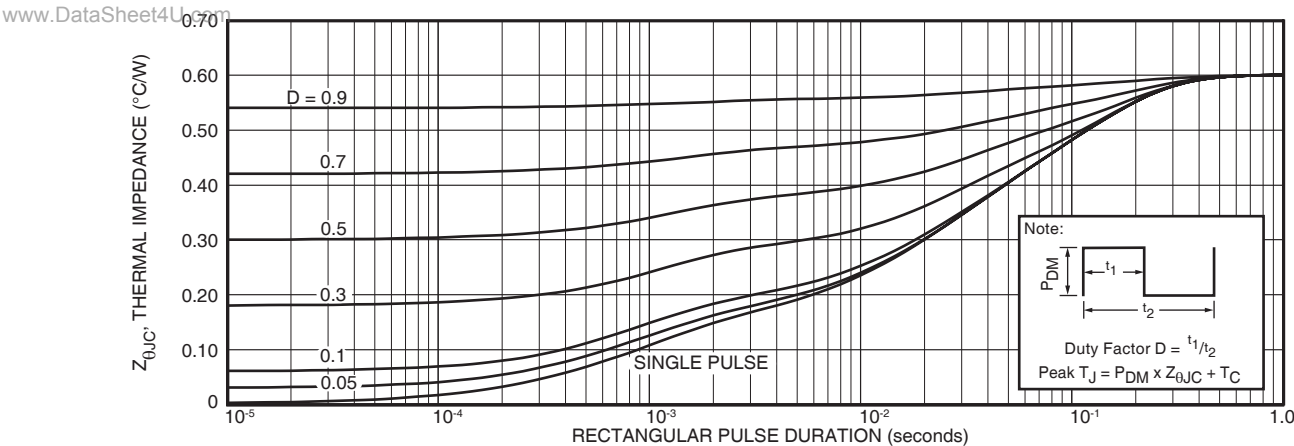
FIGURE 24a. MAXIMUM EFFECTIVE TRANSIENT THERMAL IMPEDANCE, JUNCTION-TO-CASE vs. PULSE DURATION
