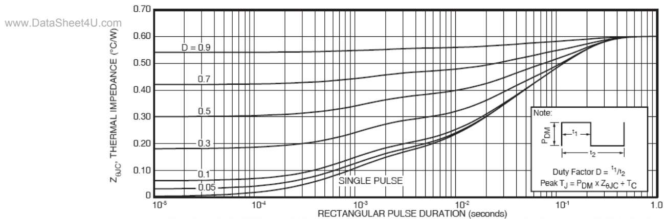
FIGURE 1a. MAXIMUM EFFECTIVE TRANSIENT THERMAL IMPEDANCE, JUNCTION-TO-CASE vs. PULSE DURATION
