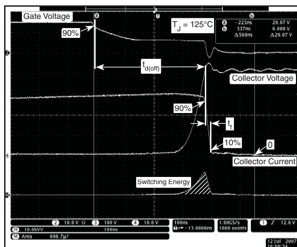
Figure 24, Turn-off Switching Waveforms and Definitions
