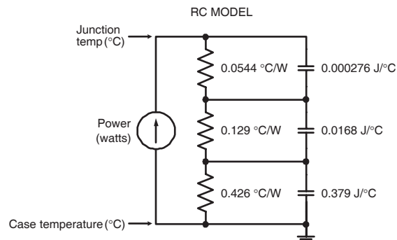
FIGURE 1b. TRANSIENT THERMAL IMPEDANCE MODEL
