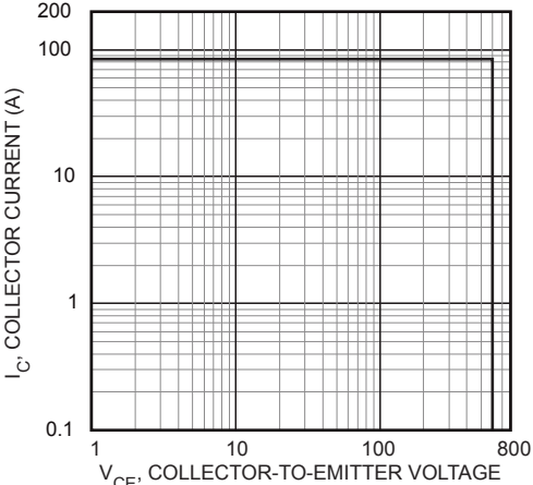
FIGURE 18, Minimum Switching Safe Operating Area
