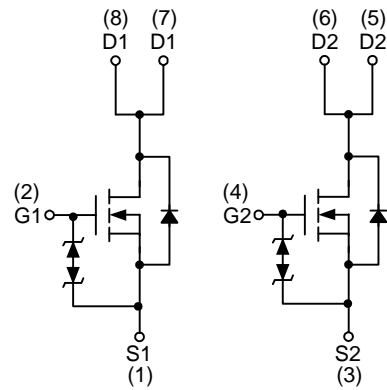
N-Channel MOSFET
