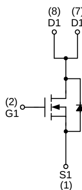
N-Channel MOSFET
