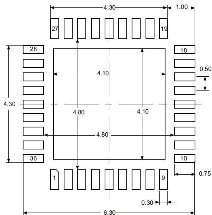
Figure 30 QFN36 - 36 Pins, 6 x 6mm Welding Layout Recommendations
