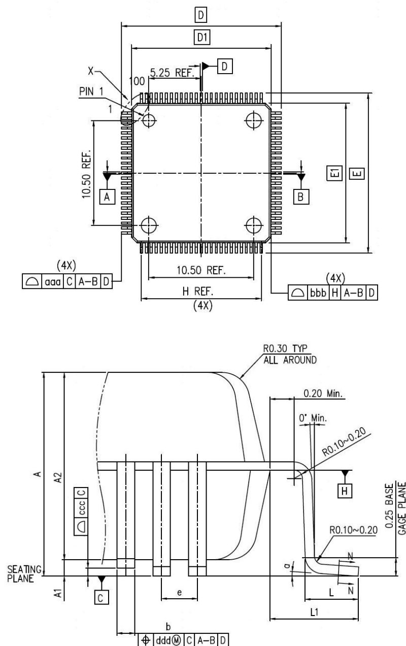
Figure 20LQFP100 Package Diagram
