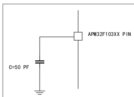
Figure 8 Load conditions when measuring pin parameters
