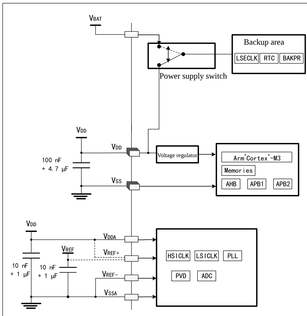
Figure 7 Power Supply Scheme
