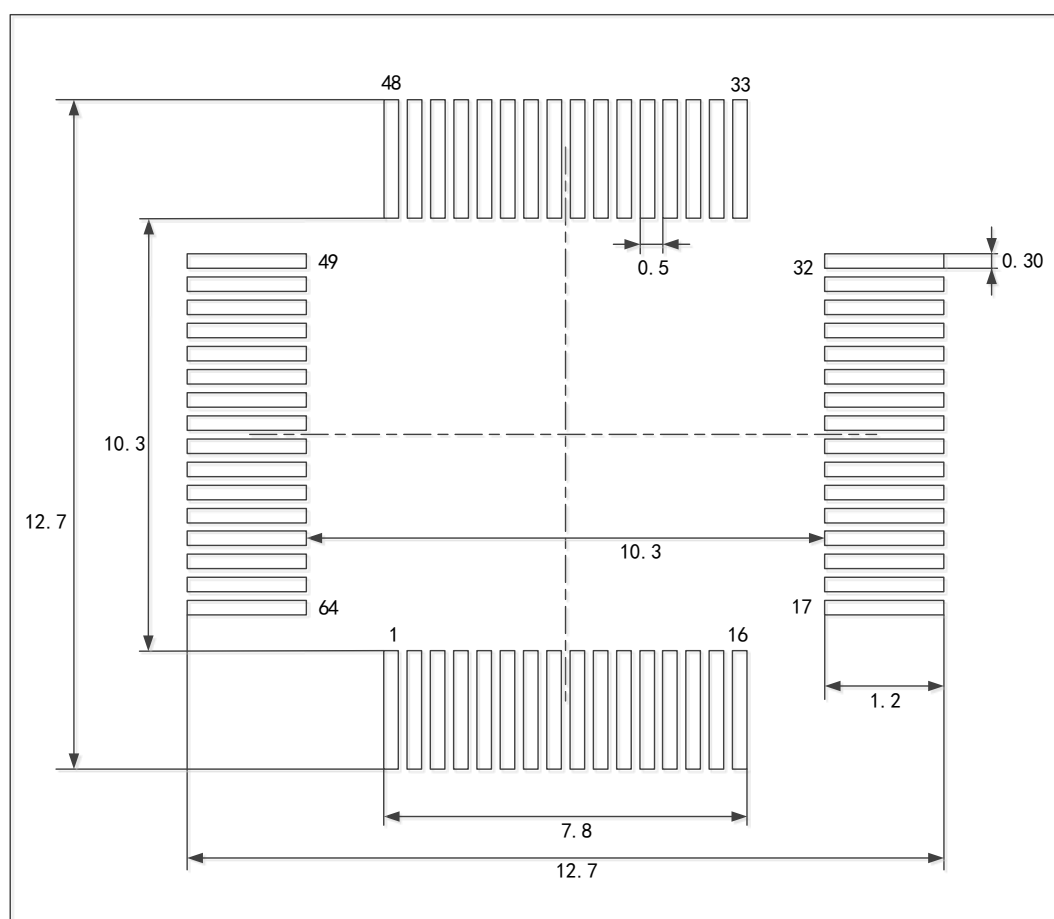
Figure 18 LQFP64 Recommended Welding Layout
