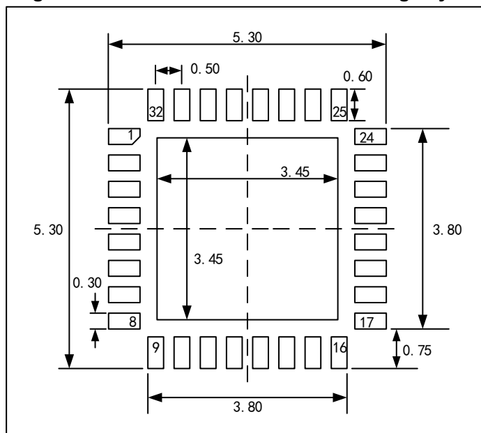
Figure 29 QFN32 Recommended Welding Layout
