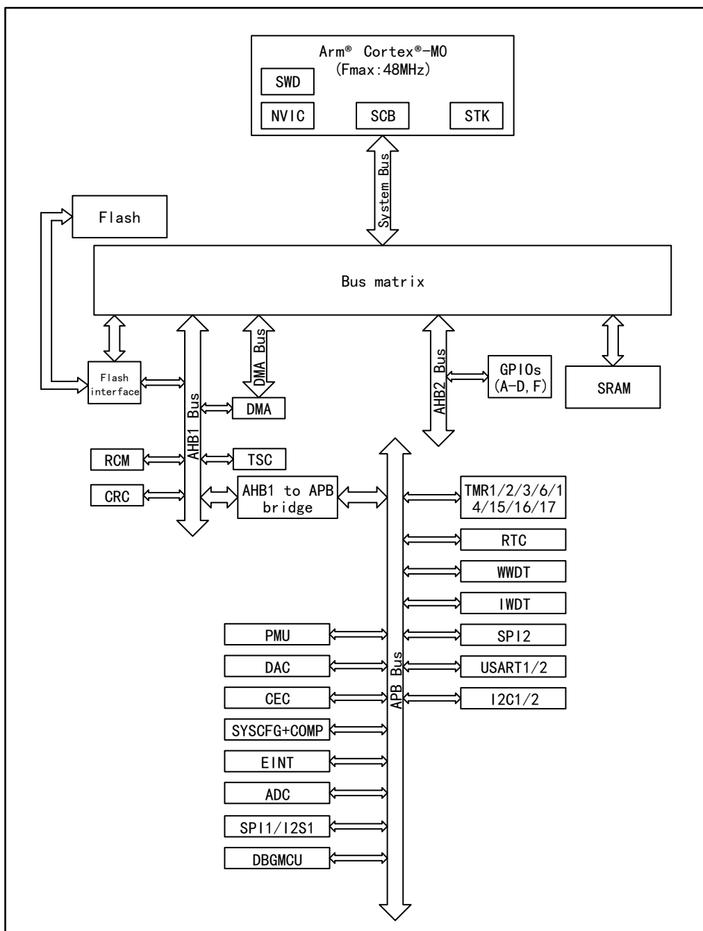
Figure 6 System Block Diagram
