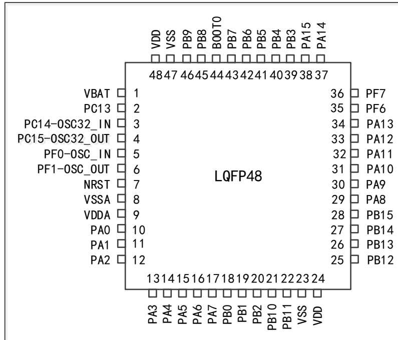
Figure 2 Distribution Diagram of APM32F051x6x8 Series LQFP48 Pins
