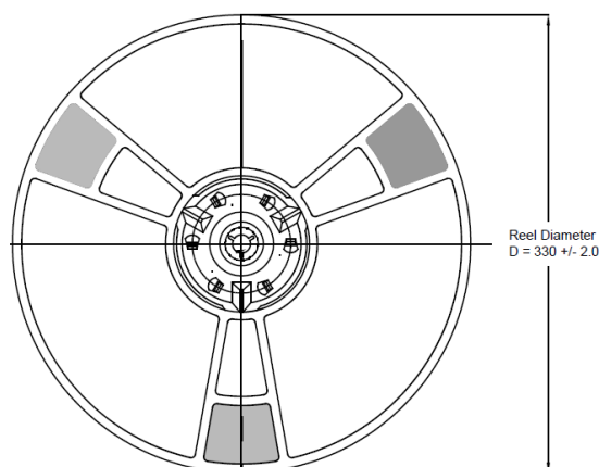
Figure 17 Reel Dimensions
