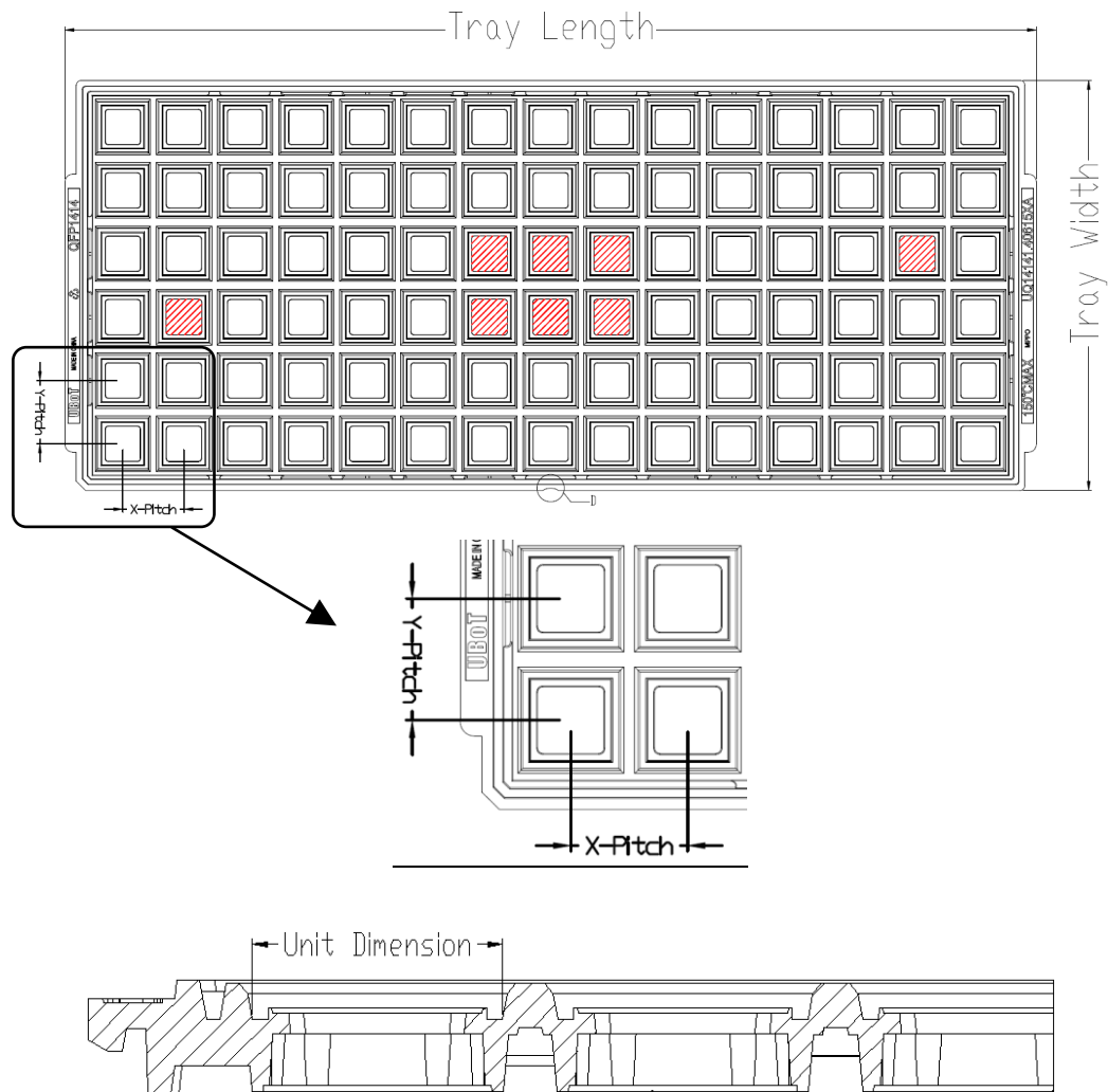
Figure 19 Tray Dimensions
