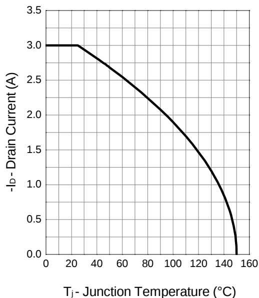
Drain Current
