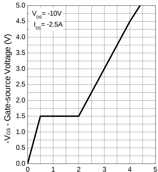
Gate Charge
