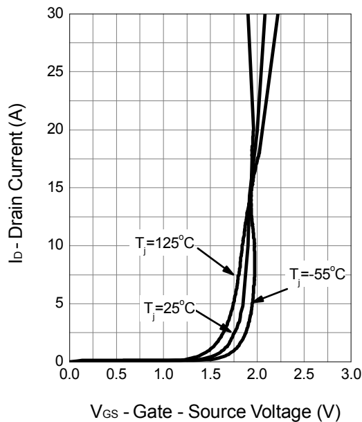
Transfer Characteristics
