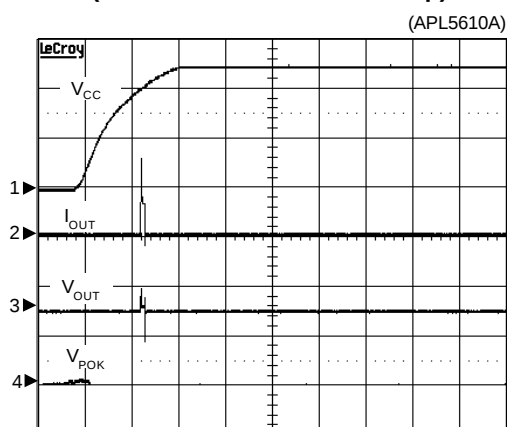
Short Circuit Response (Short-Circuit before Power-up)
