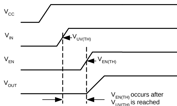
Figure 1. APL5610A supply comes up before MOSFET drain supply
