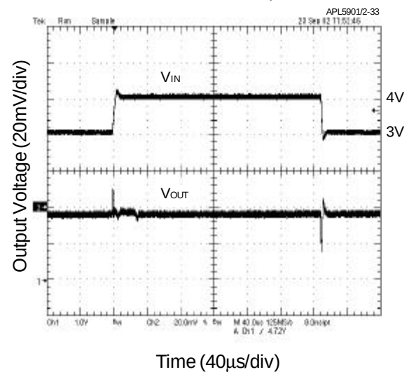
Line-Transient Response
