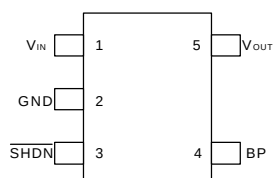
SOT-23-5 (Top View)
