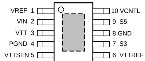
MSOP-10P (Top View)
