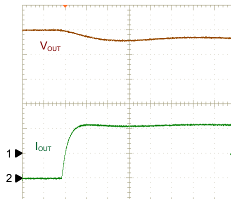
Load-Transient Response
