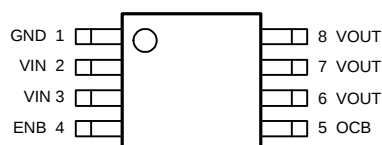
SOP-8/MSOP-8 APL3550B/D (Top View)
