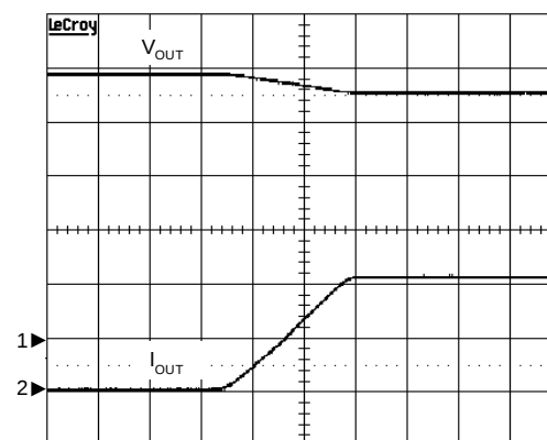
Load-Transient Response
