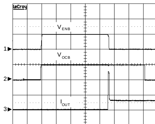
OCB Response During Over Load
