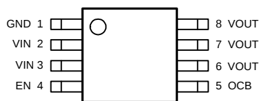
SOP-8/MSOP-8 APL3550A/C (Top View)
