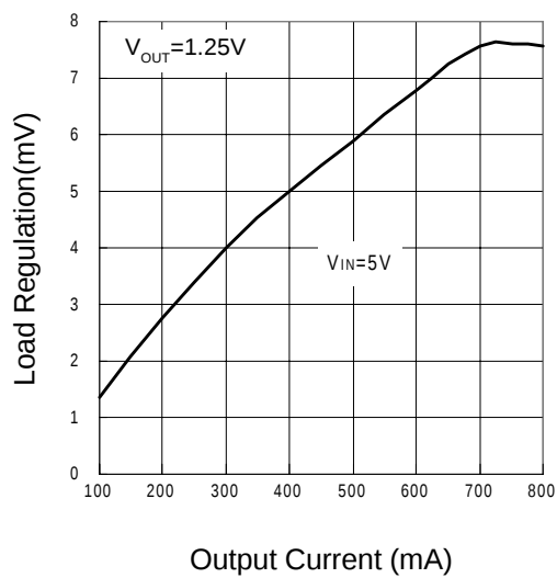
Load Regulation vs. Output Current
