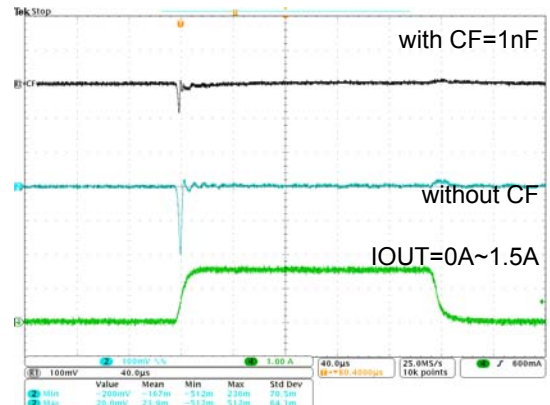
Fig.2 Load Transient, 3Vi to 1.8Vo
