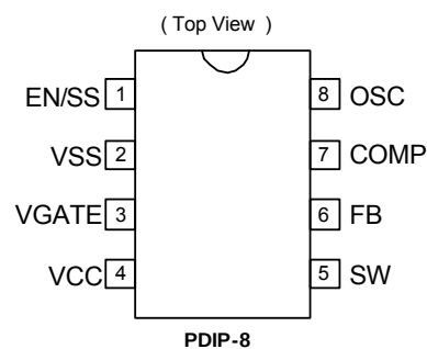
PDIP-8
