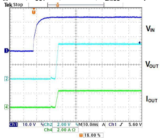
Power-ON Wave (F=60KHz) ( V_{IN}=24V , V_{OUT}=5V , Load=2A, C_{EN/SS}=0.1\mu F )
