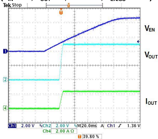
Enable-ON Wave (60KHz) ( V_{IN}=12V , V_{OUT}=5V , Load=2A, C_{EN/SS}=0.1\mu F )
