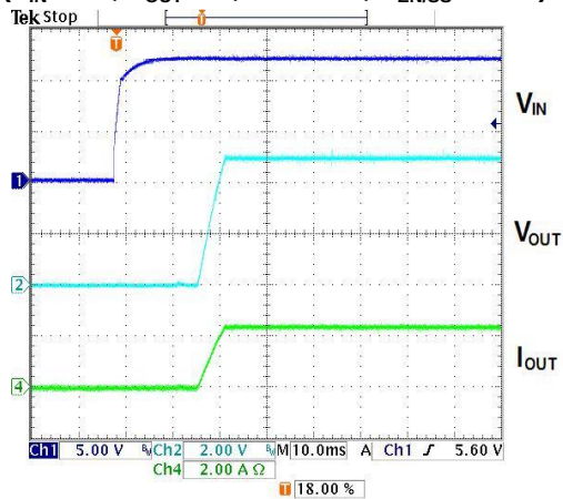
Power-ON Wave (F=60KHz) ( V_{IN}=12V , V_{OUT}=5V , Load=2A, C_{EN/SS}=0.1\mu F )
