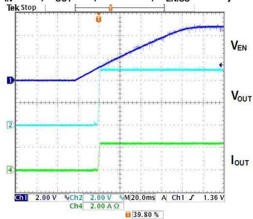
Enable-ON Wave (60KHz) ( V_{IN}=24V , V_{OUT}=5V , Load=2A, C_{EN/SS}=0.1\mu F )
