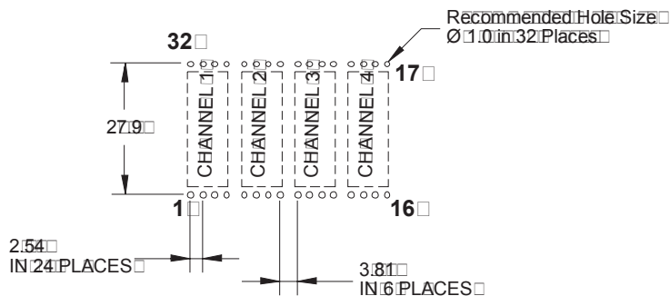
Recommended P.C.B Pad Layout
