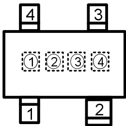
SC-82 (I) (Top View)
