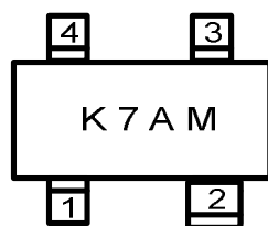
SC-82 (I) (Top View)
