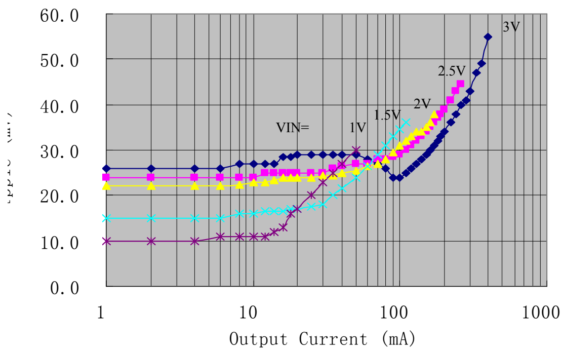
Output Current VS. Ripple
