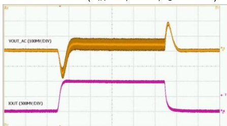
Load Transient (V IN =3V, PWM, I O =0 to 1A)
