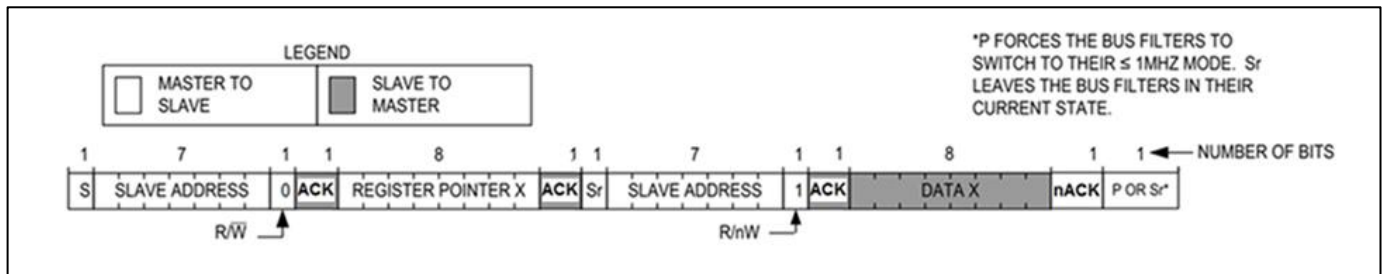
Figure 9. Reading from a Single Register X
