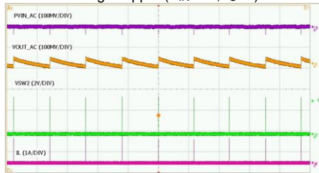
Voltage Ripple (V IN =3V, I O =0)
