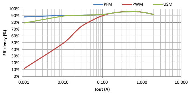
Efficiency, P VIN =3.3V, V OUT =3.4V
