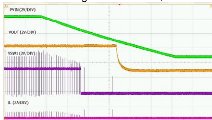
Shutdown through P VIN No Load, V IN =5.5V
