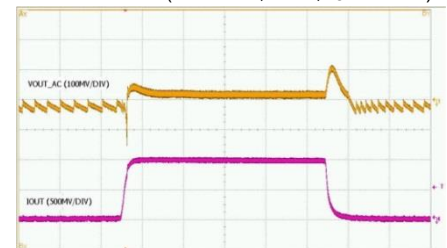
Load Transient (V IN =5.5V, PFM, I O =0 to 1A)
