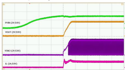
Startup through P VIN 1A Load, V IN =3V
