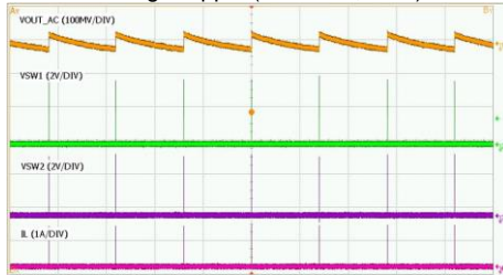
Voltage Ripple (V IN =3.8V, I O =0)
