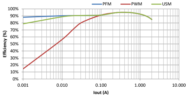
Efficiency, P VIN =2.7V, V OUT =3.4V
