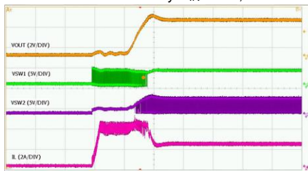
Short-Circuit Recovery V IN =3.8V, 2A Load
