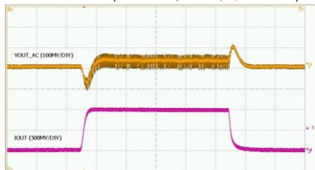
Load Transient (V IN =3.8V, PWM, I O =0 to 1A)
