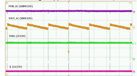
Voltage Ripple (V IN =5.5V, I O =0)
