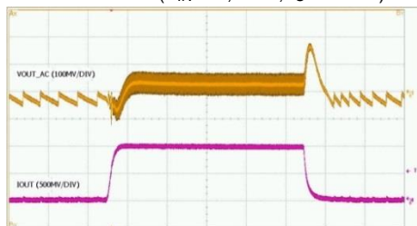
Load Transient (V IN =3V, PFM, I O =0 to 1A)
