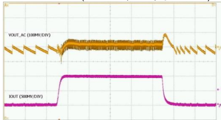
Load Transient (V IN =3.8V, PFM, I O =0 to 1A)
