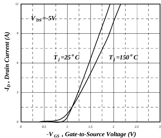
Fig 11. Transfer Characteristics
