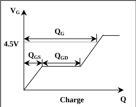
Fig 12. Gate Charge Waveform
