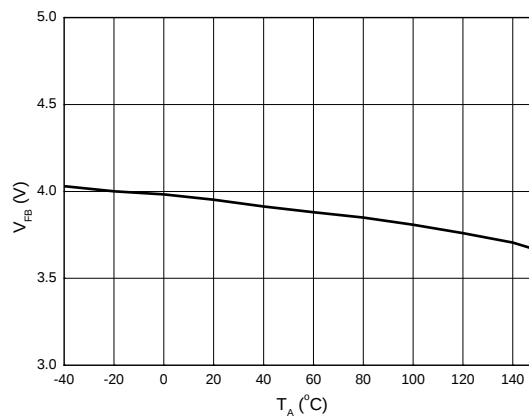
V_{FB} vs. T_A
