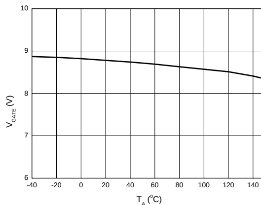
V_{GATE} vs. T_A
