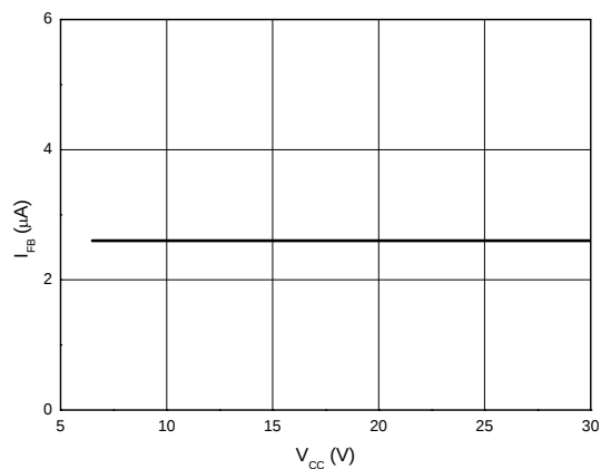
I_{FB} vs. V_{CC}
