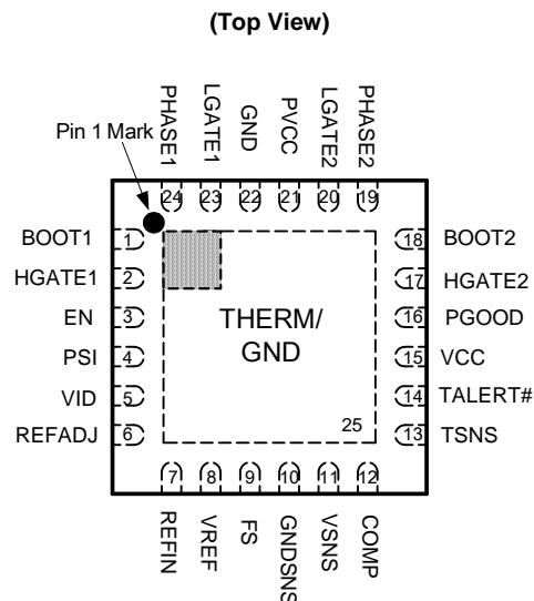
U-QFN4040-24
