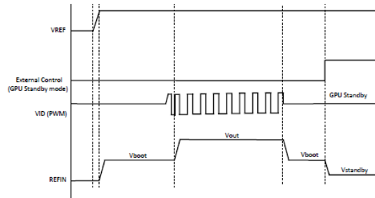
Figure 8. Time Diagram
