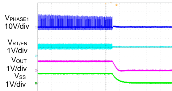
Power Off Waveforms
