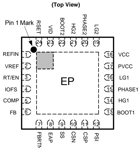
U-QFN4040-24 (FN Package)
