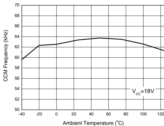
CCM Frequency vs. Ambient Temperature
