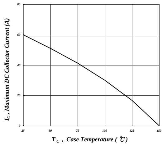
Fig 13. Collector Current VS. Case Temperature
