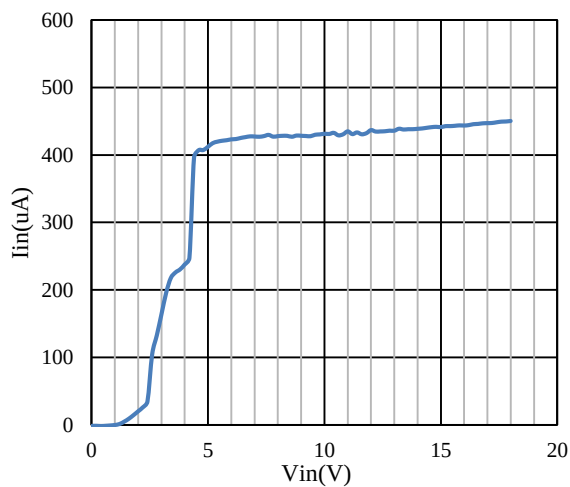
Figure 5. Input current vs. Input voltage
