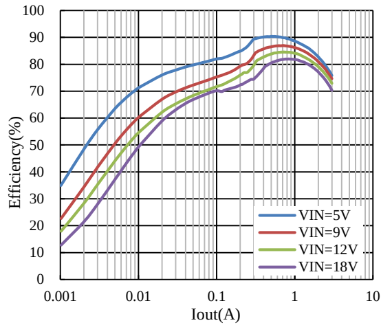
Figure 1. Efficiency vs. Load Current, V_{OUT} = 1.2V
