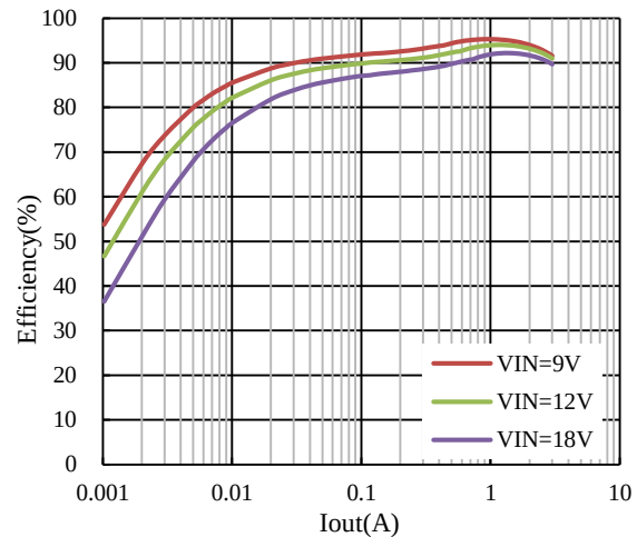
Figure 4. Efficiency vs. Load Current, V_{OUT} = 5V
