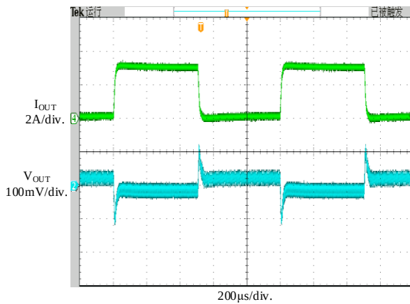
Figure 11. Load Transient, V_{OUT}=3.3V , I_{OUT}=0.1A-3A
