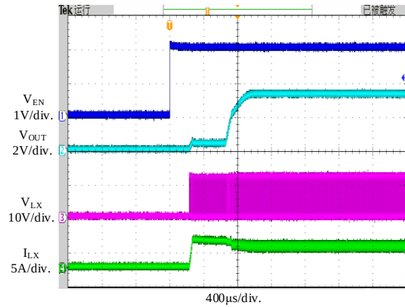
Figure 7. Startup Waveforms
