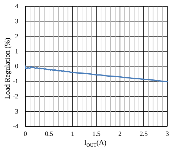
Figure 6. Load Regulation vs. Load Current
