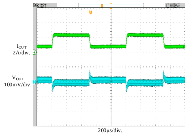
Figure 12. Load Transient, V_{OUT}=3.3V , I_{OUT}=0.75A-2.25A
