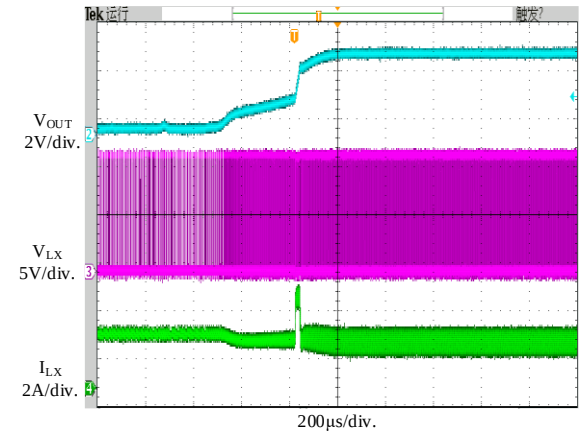
Figure 10. Short Circuit Recovery
