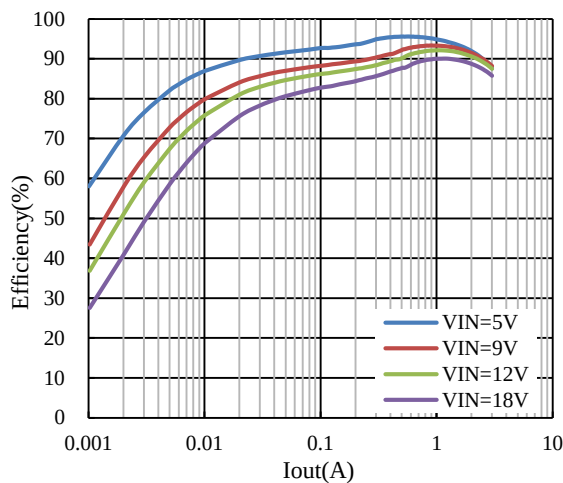
Figure 3. Efficiency vs. Load Current, V_{OUT} = 3.3V
