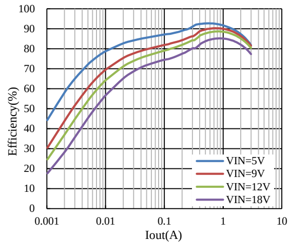
Figure 2. Efficiency vs. Load Current, V_{OUT} = 1.8V
