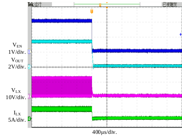
Figure 8. Shutdown Waveforms
