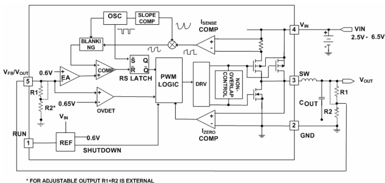
Figure 3. AP2406 Block Diagram
