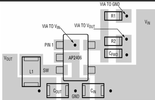
Figure4. AP2406 ADJ output Suggested Layout
