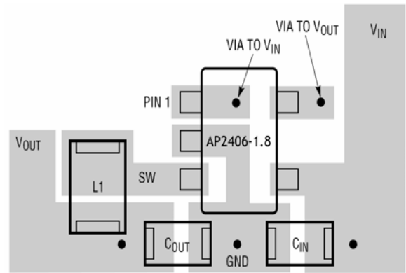
Figure5. AP2406 Fixed output Suggested Layout
