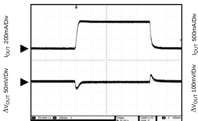
Figure 12. Load Transient Response V_{IN}=2.5V , V_{OUT}=1.25V , I_{OUT}=1 to 500mA , C_{IN}=1\mu F , C_{OUT}=2.2\mu F
