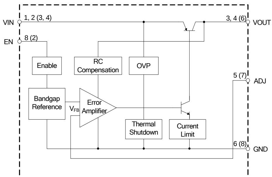
Figure 3. Functional Block Diagram of AP2318A
