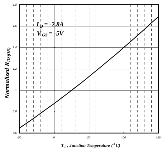
Fig 4. Normalized On-Resistance
