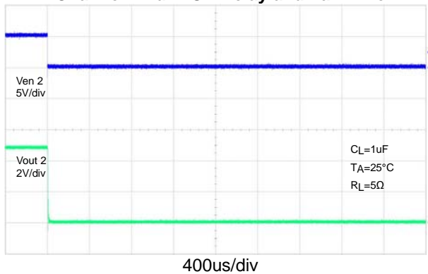
Channel 2 Turn-Off Delay and Fall Time
