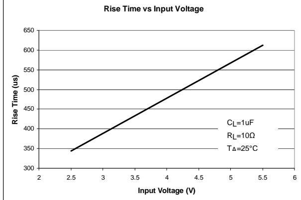
Rise Time vs Input Voltage
