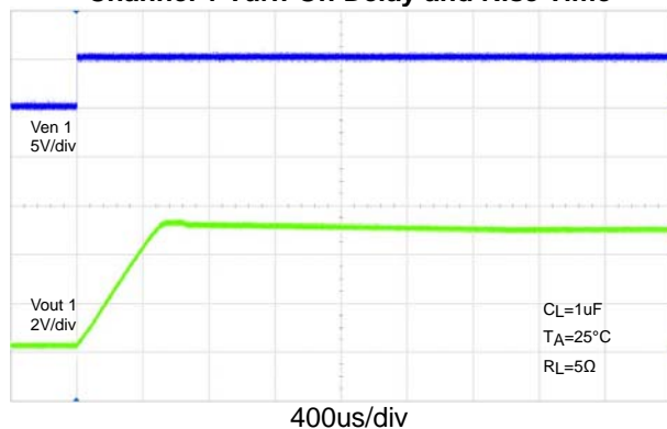
Channel 1 Turn-On Delay and Rise Time
