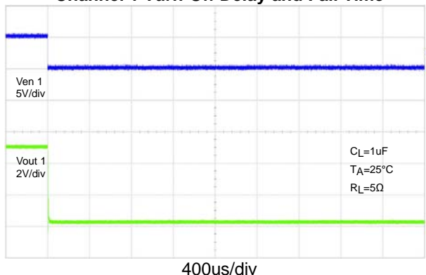
Channel 1 Turn-Off Delay and Fall Time
