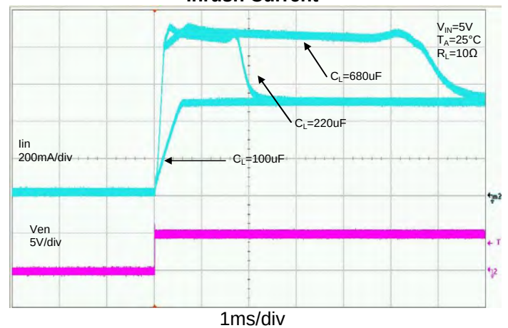
Inrush Current
