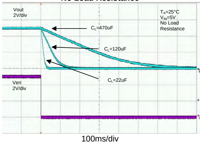
Discharge Time No Load Resistance
