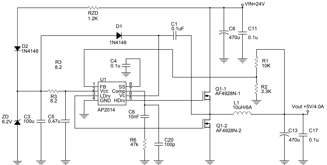
Single Supply 24V Input
