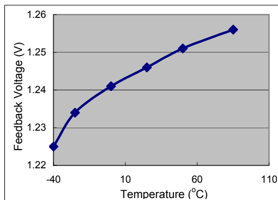
Feedback Voltage v.s. Temperature Vin=5V; Vout=15V
