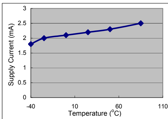
Supply Current v.s. Temperature Vin=5V; Vout=15V; Iout=0A
