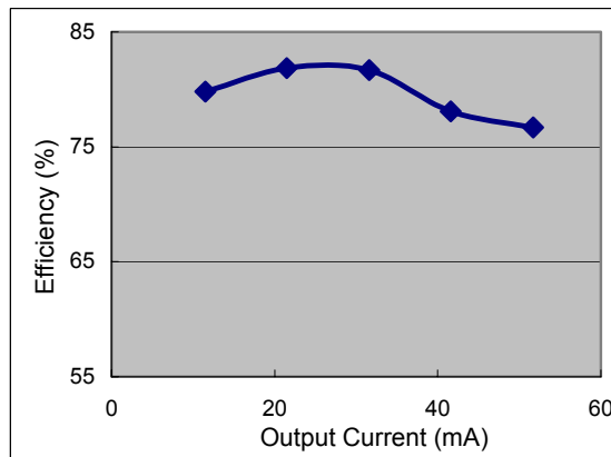
Efficiency v.s. Output Current Vin=3.3V; Vout=15V
