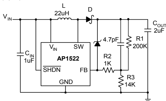
Figure 1. With Open-Circuit Protection
