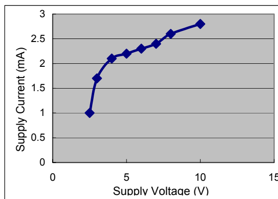
Supply Current v.s. Supply Voltage Vout=15V; Iout=0A
