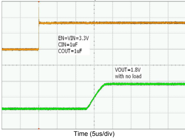
Start-up Time
