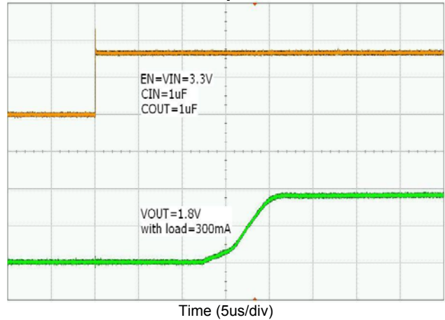
Start-up Time
