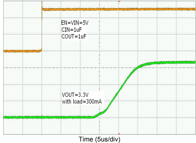
Start-up Time
